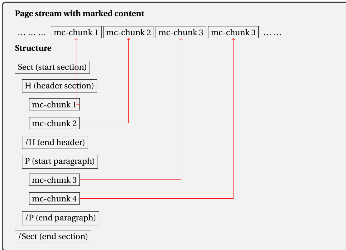
Figure 4: Schematical description of the relation between marked content in the page stream and the structure
